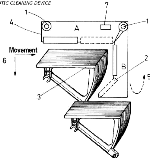
ESCALATOR ROBOTIC CLEANING DEVICE
